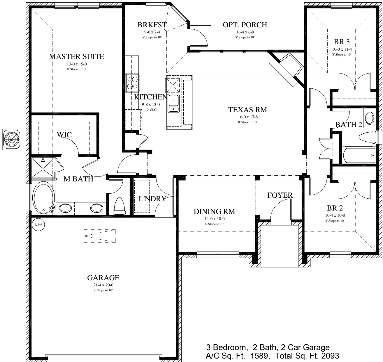
FLOOR PLAN
